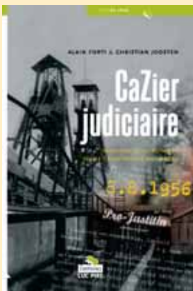
Cazier judiciaire,
